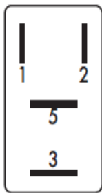
Micro relay terminal configuration
