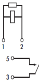
Micro relay terminal configuration
